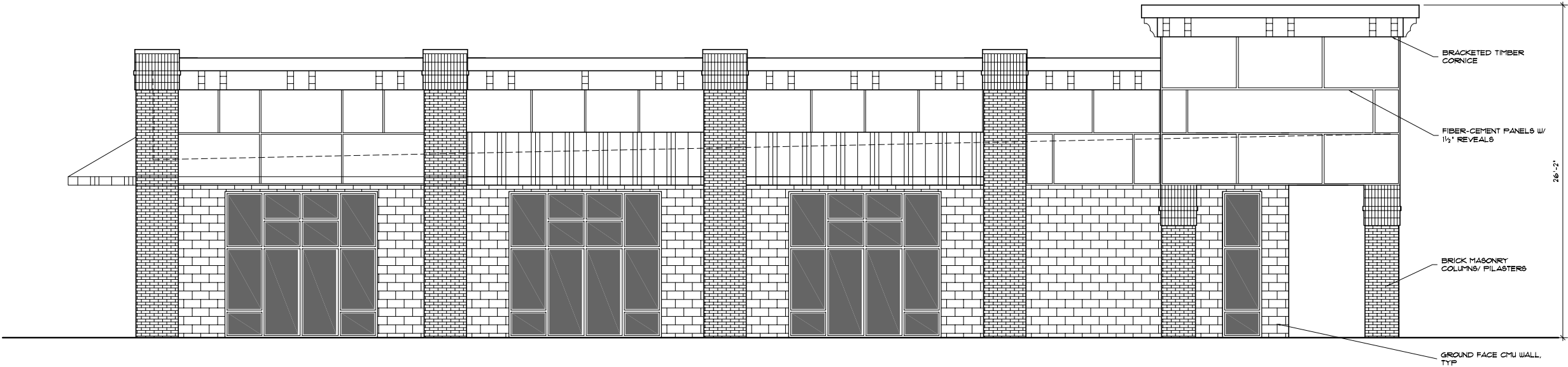
NORTHEAST ELEVATION
